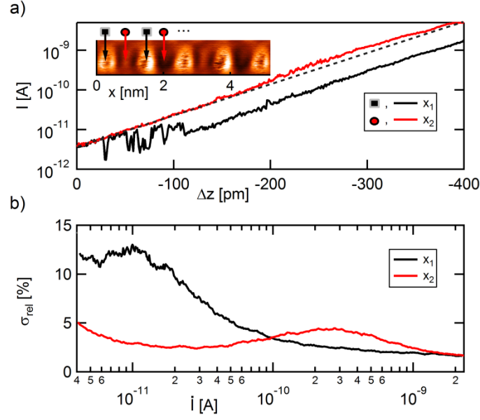
FIG.5: a): Typical I(z) curves ( U_{\text{gap}} = 1.3 V, T = 57 K) measured over a bright 1 \times 3 protrusion (black; position x_1 ) and in between (red; position x_2 ), respectively. The dotted line is a guide to the eye representing a purely exponential behavior. Inset: topography ( U_{\text{gap}} = 1.3 V, I = 10 pA, T = 60 K) of a single Si step-edge showing a 1 \times 3 periodicity and the locations of x_1 and x_2 . Fluctuations on top of bright 1 \times 3 protrusions can be seen as dark horizontal stripes. b): The relative standard deviation of the tunneling current as a function of the mean current measured on positions x_1 and x_2 . The curves represent an average over \sim 200 measurements. The peaks in the relative standard deviation reveal the typical currents where the 1 \times 3 \leftrightarrow 1 \times 2 structural fluctuations occur and show that at these currents differ for the two locations x_1 and x_2 .
